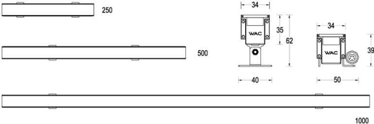
Line Drawing
