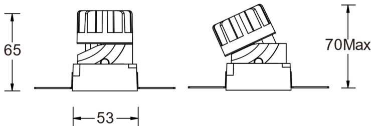
Line Drawing
